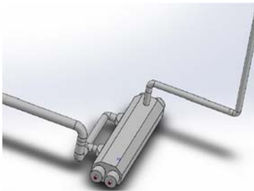
Figure 2 Solidworks Drawing of Pyrolysis Process
