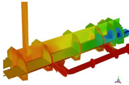
Figure 1 Computational Fluid Dynamics Modelling of Temperature Profile
