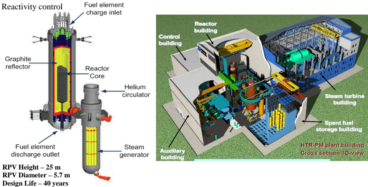
Figure 5.1-6. Conceptual Drawing of HTR-PM Reactor System and 2-Unit Plant Configuration
