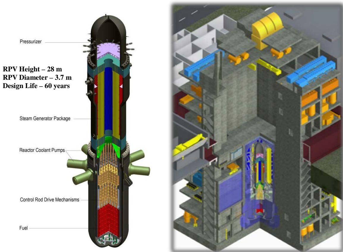
Figure 3-8. Conceptual Drawing of the Westinghouse SMR Reactor Module and Plant
