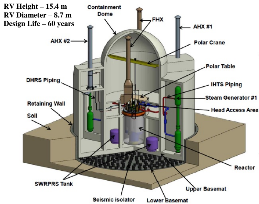
Figure 7.4-2. Conceptual Drawing of the PGFSR Plant Configuration
