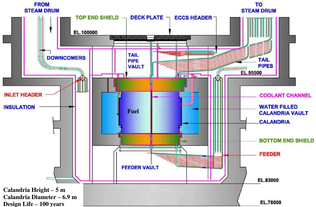
Figure 4-1. Conceptual Drawing of the AHWR300-LEU Reactor
