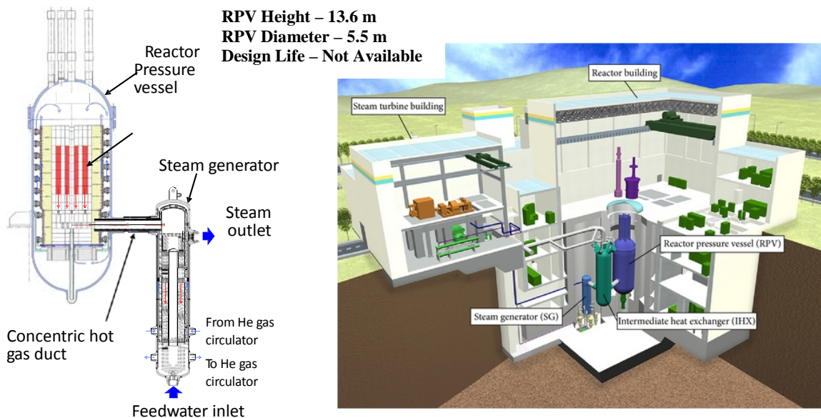
Figure 5.1-4. Conceptual Drawing of HTR50S Reactor System and Plant Configuration
