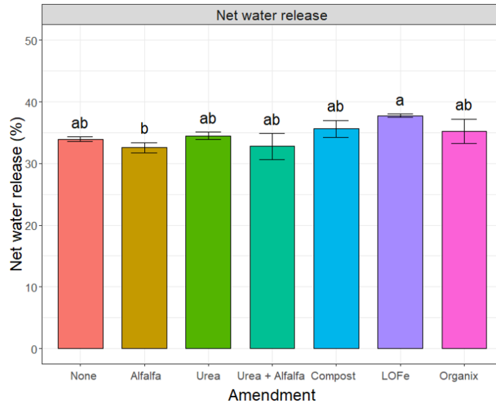
Figure 2: Comparison of average NWR% between chosen additives, added to SFR 0.0 before flocculation. Error bars represent one standard error of the mean ( \pm SE, n = 4 ). Different letters indicate a significant difference ( p < 0.05 ) amongst amendment type.
