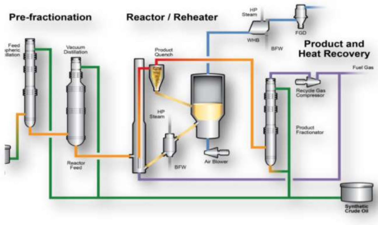
Figure 5.8: HTL Process Flow Schematic
