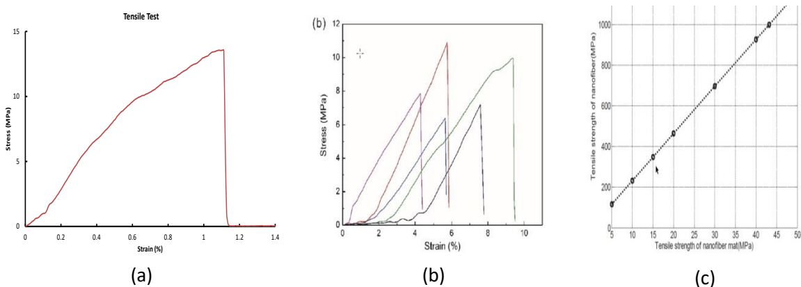
Fig. 5 (a) Stress-strain curves of PAN/AOA CF mats; (b) Stress-strain curves of PAN CF mats; (c) Predicted tensile strength of individual nanofibre vs. the tensile strength of nanofibre mats
